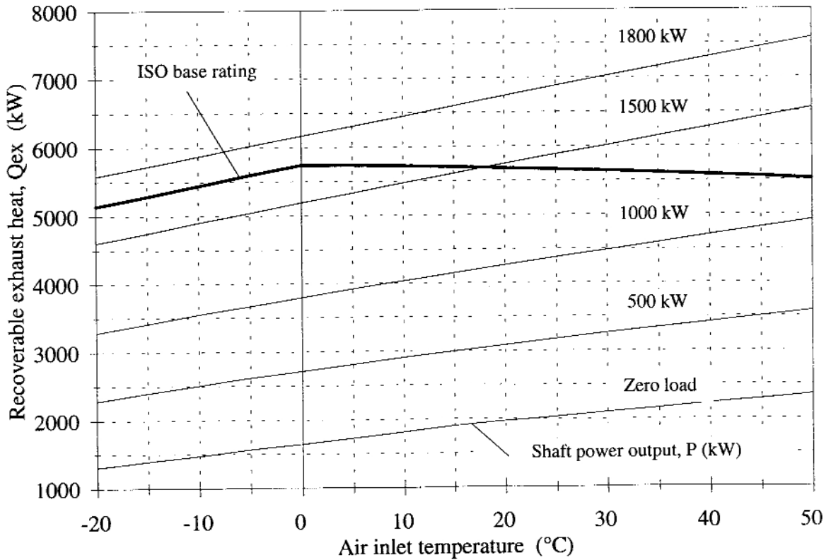
Figure 3: Recoverable exhaust heat (referred to 160°C) vs. gear shaft power output and air inlet temperature
